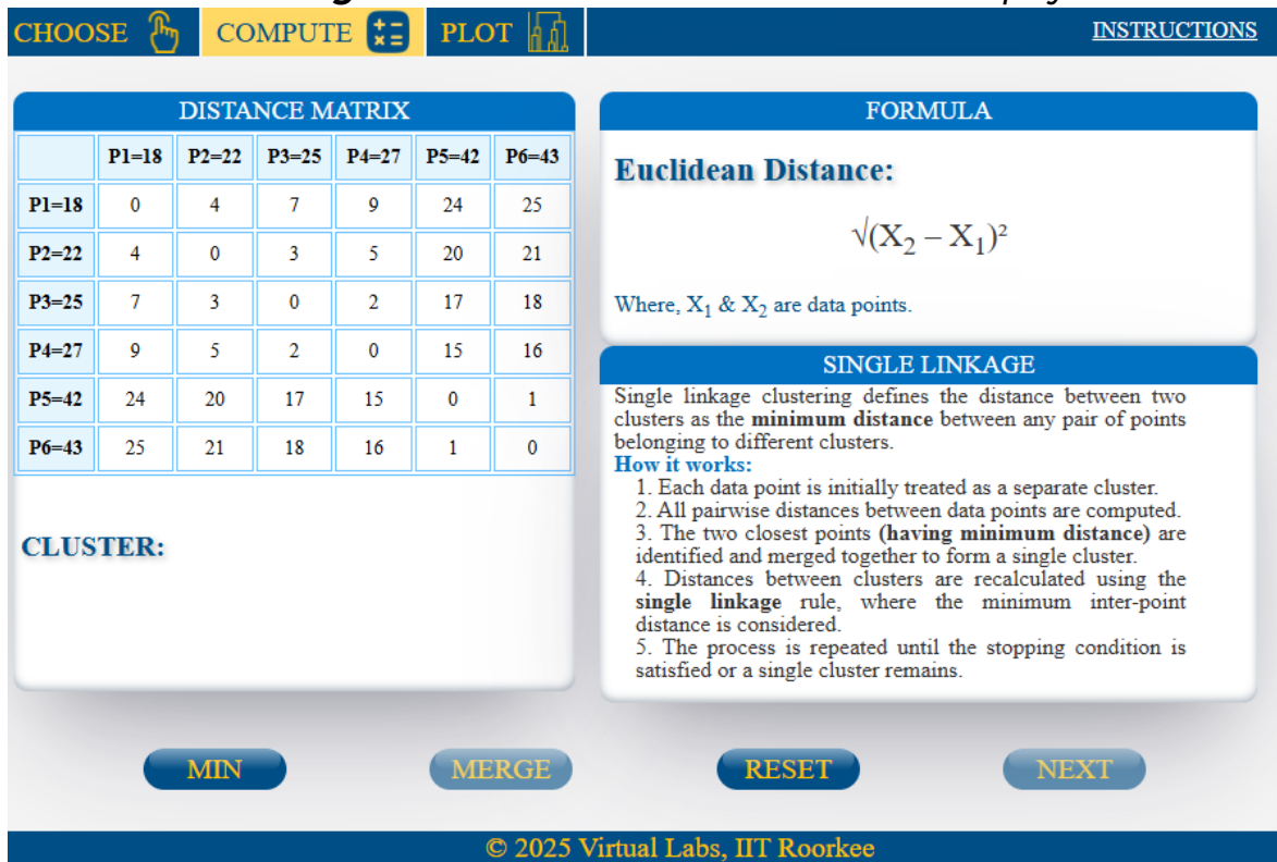
Fig 4: Calculated distance matrix for all data points
